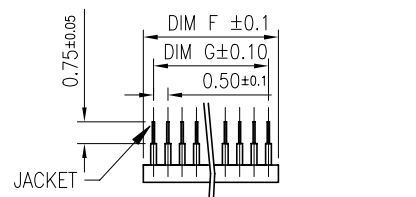
RECOMMENDED DISCRETE. CABLE Dimension
