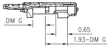
SECTION A-A SCALE 8:1
