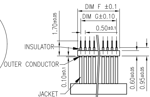
RECOMMENDED SGC CABLE Dimension
